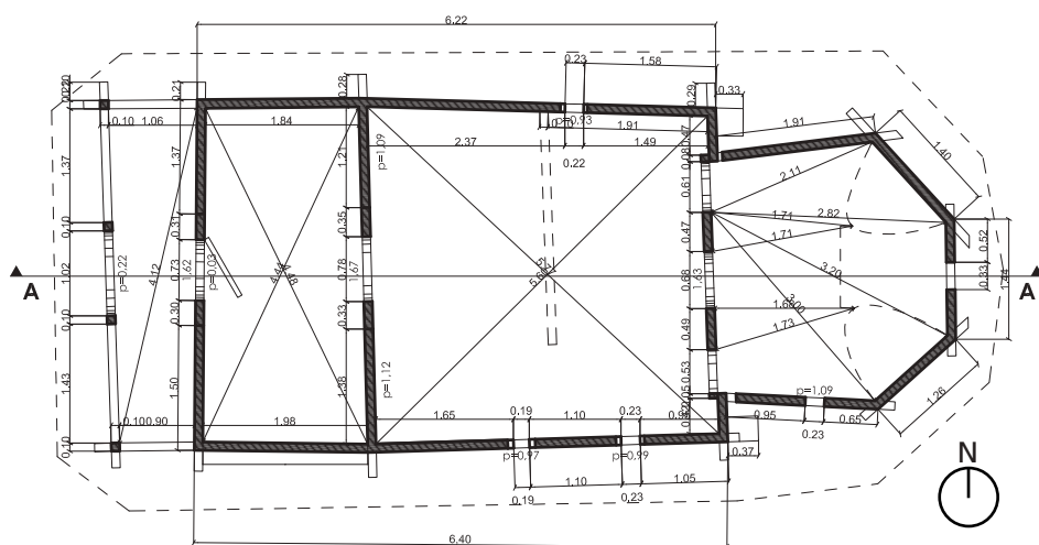
Plan sc. 1:100
