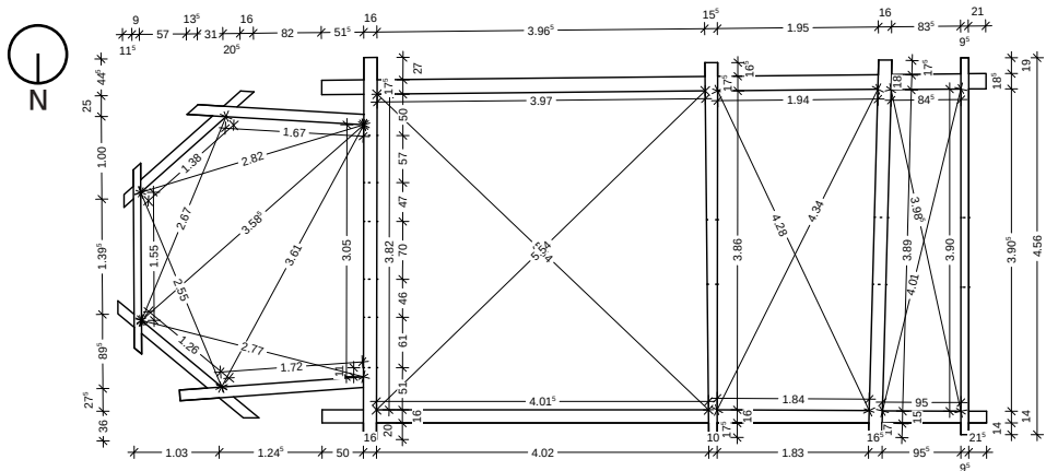
Plan tălpi
