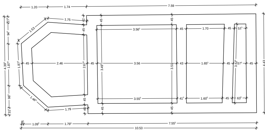
Plan soclu
